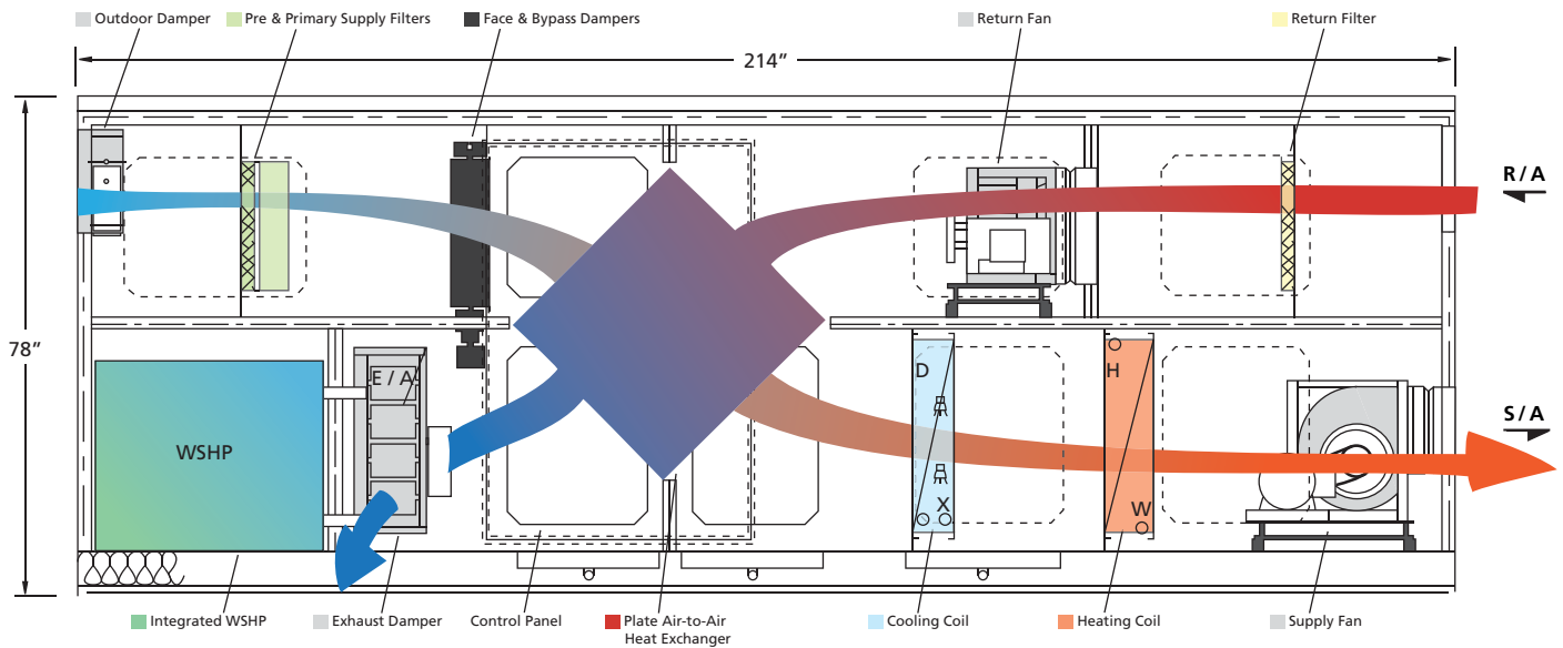
Elevation view of a Venmar CES EnergyPack® air handler with plate energy recovery heat exchanger, and with integrated water source heat pump, shown in winter operating mode.
